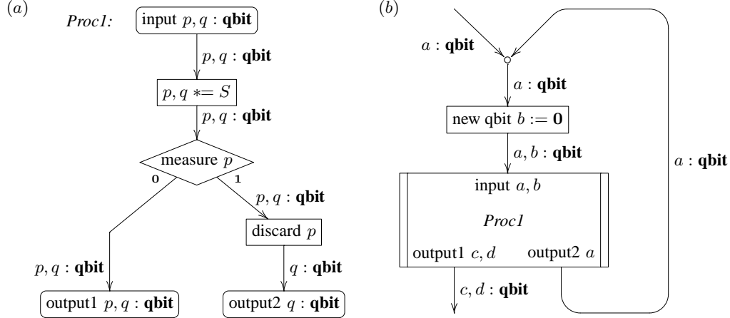
Fig. 6. A procedure and a procedure call
