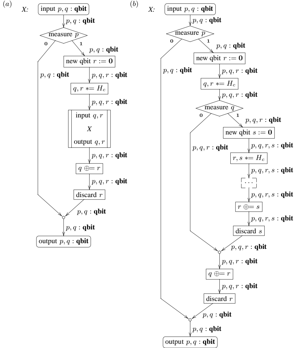
Fig. 8. A recursive procedure and its unwinding
