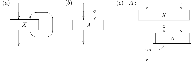
Fig. 9. Loops from recursion
