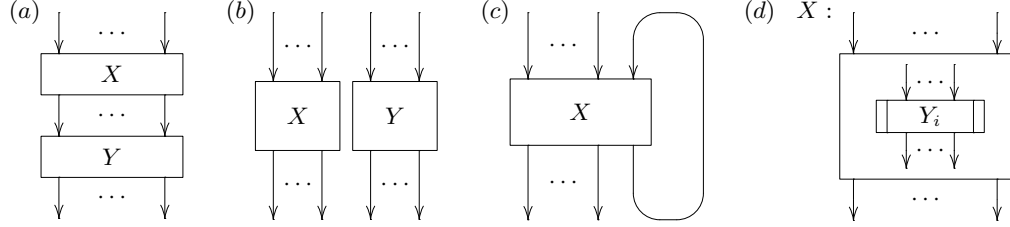
Fig. 10. Some composite flow charts
