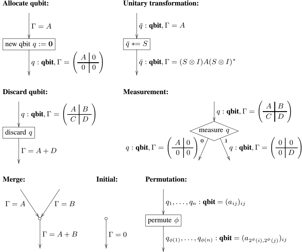
Fig. 5. Rules for quantum flow charts
