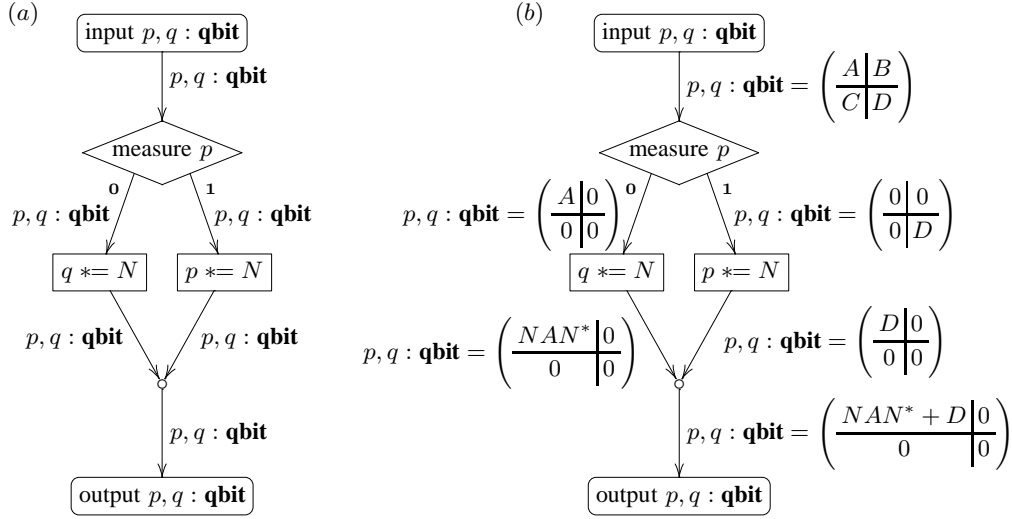
Fig. 4. A simple quantum flow chart
