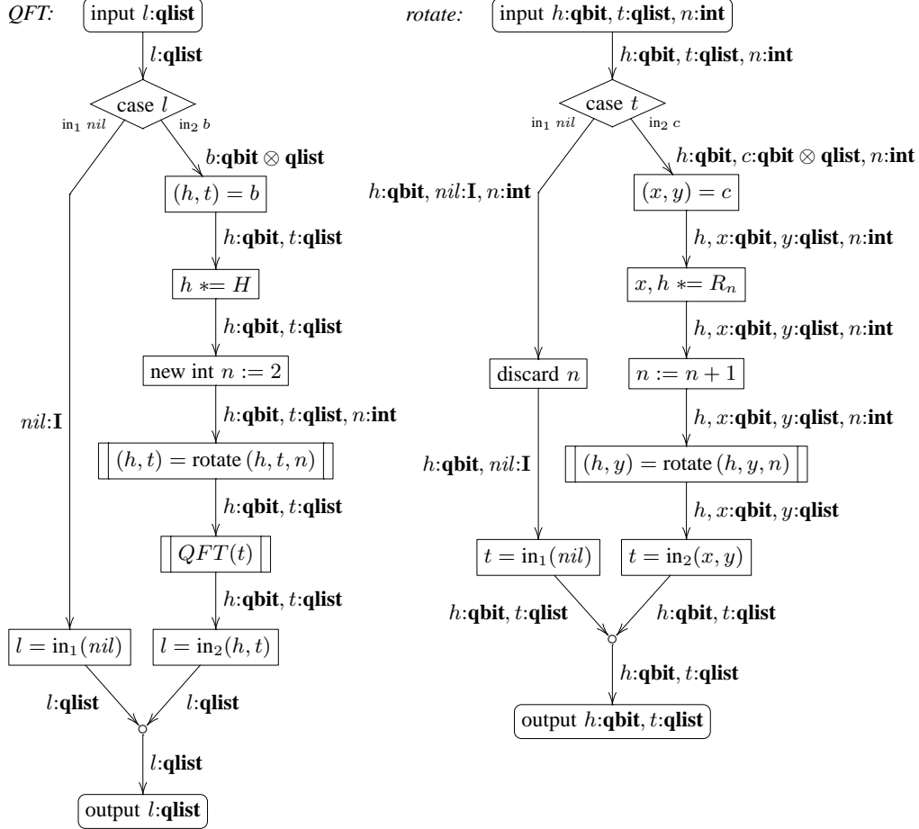
Fig. 13. The Quantum Fourier Transform
