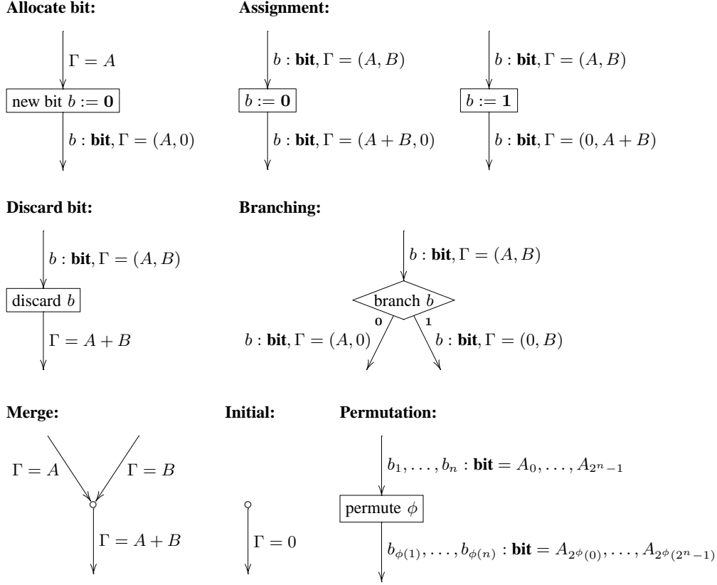
Fig. 3. Rules for classical flow charts
