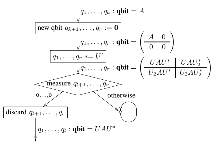
Fig. 11. Flow chart realizing a sub-unitary transformation
